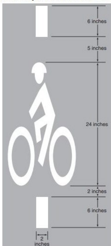
Figure 9C-7. Bicycle Detector Pavement Marking
