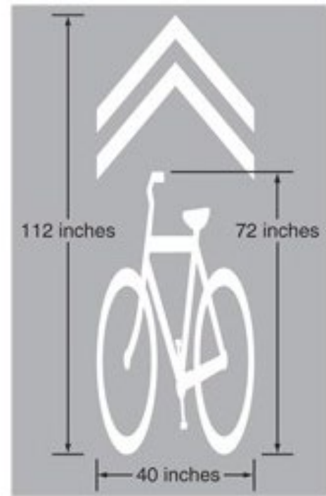
Standard Shared Lane Marking from the MUTCD.
